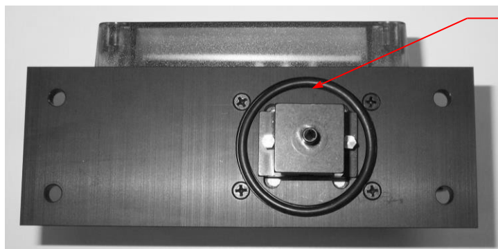
Oxygen monitor for glove box Bottom View
